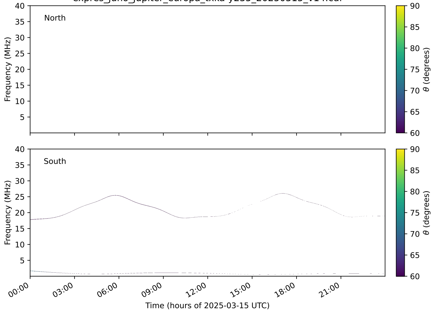
expres_juno_jupiter_europa_txka-y235_20250315_v14.cdf
