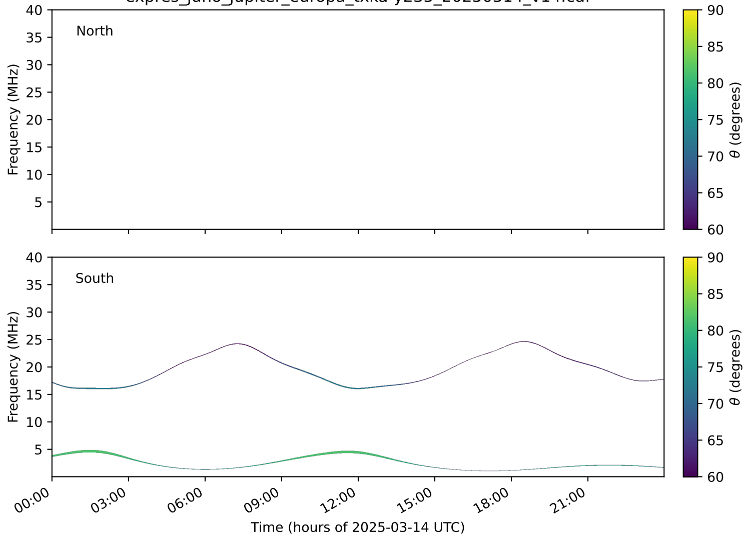
expres_juno_jupiter_europa_txka-y235_20250314_v14.cdf
