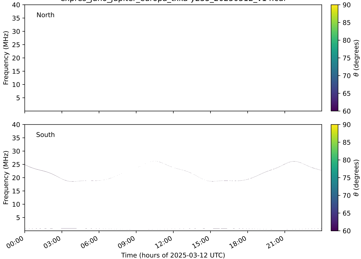
expres_juno_jupiter_europa_txka-y235_20250312_v14.cdf
