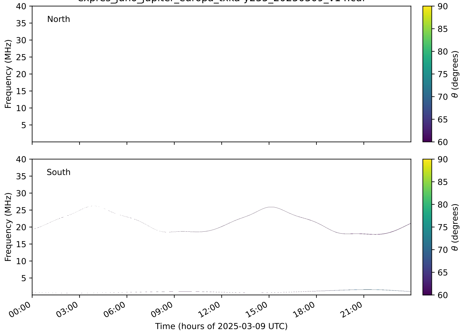
expres_juno_jupiter_europa_txka-y235_20250309_v14.cdf
