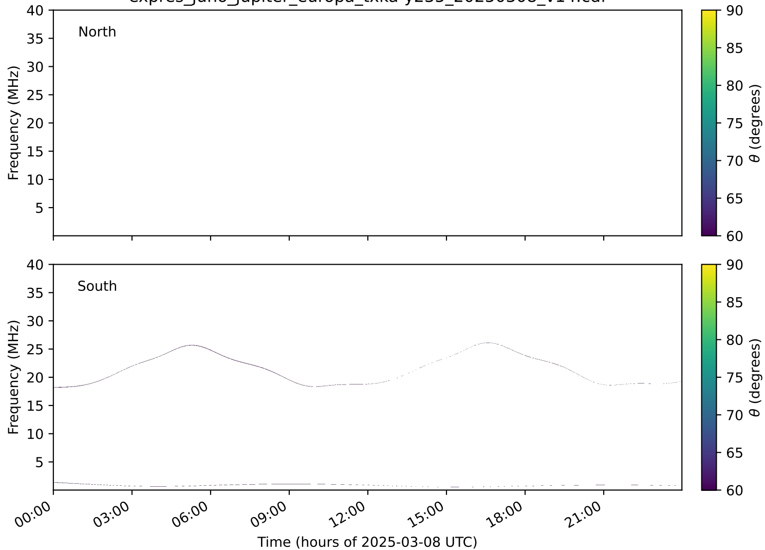
expres_juno_jupiter_europa_txka-y235_20250308_v14.cdf
