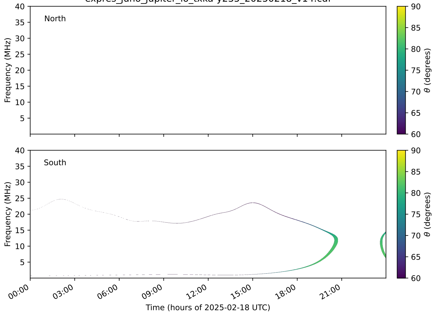
expres_juno_jupiter_io_txka-y235_20250218_v14.cdf
