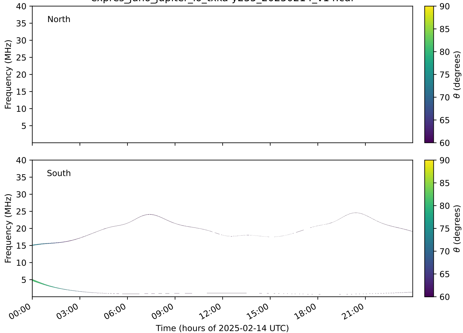
expres_juno_jupiter_io_txka-y235_20250214_v14.cdf
