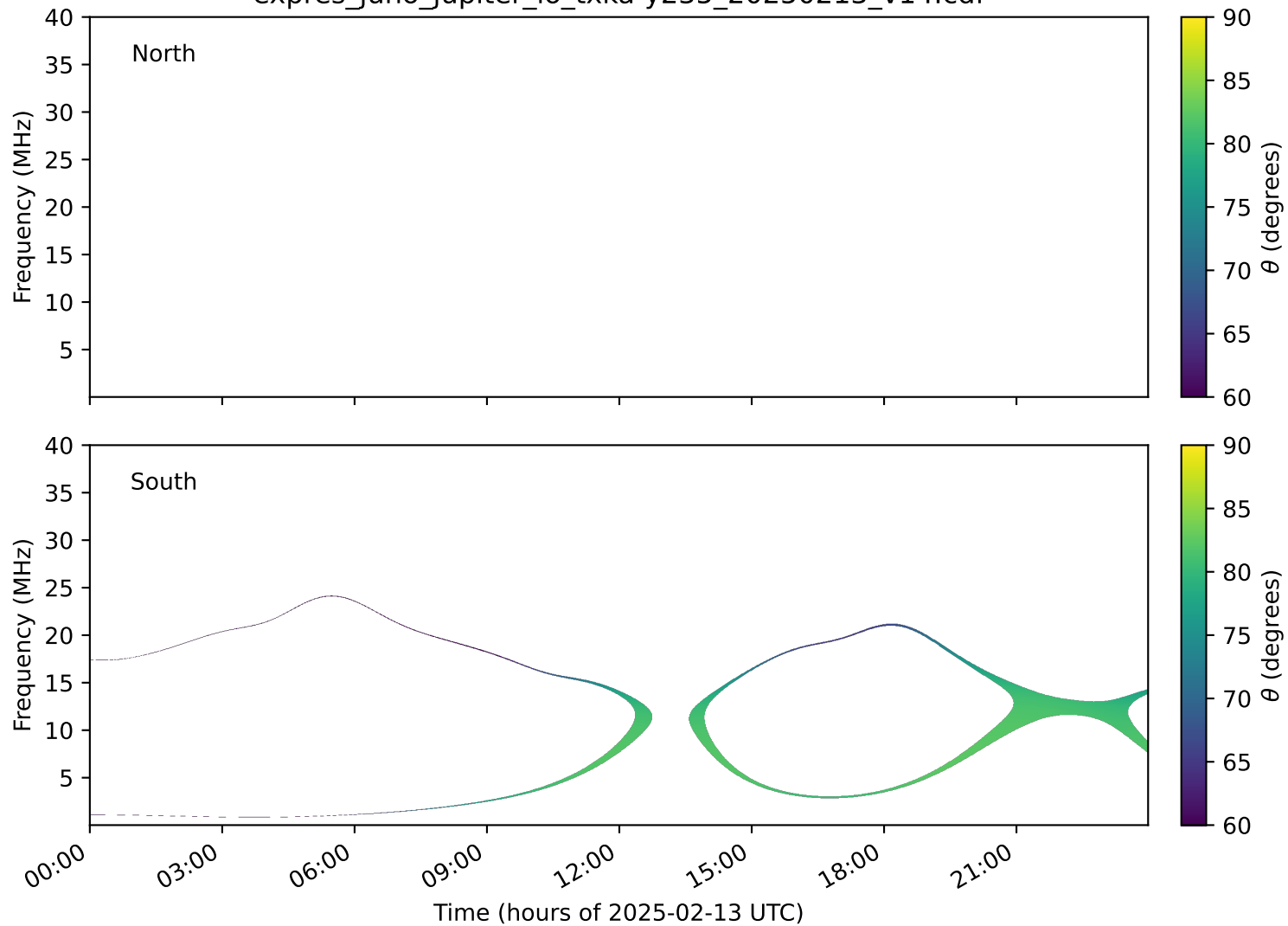
expres_juno_jupiter_io_txka-y235_20250213_v14.cdf
