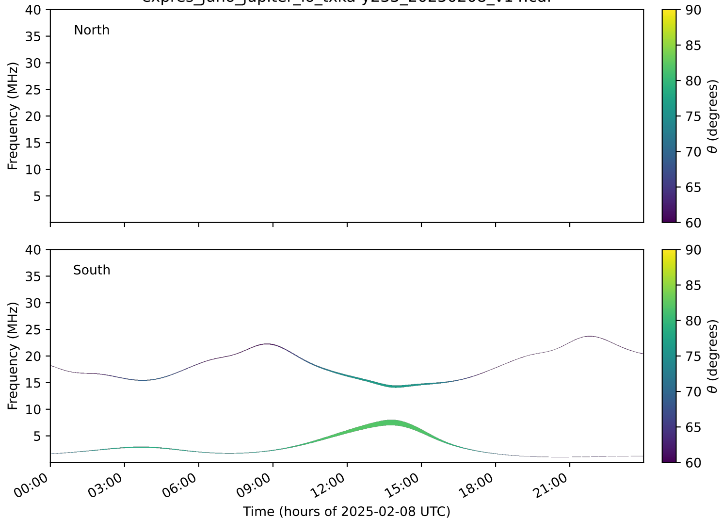
expres_juno_jupiter_io_txka-y235_20250208_v14.cdf
