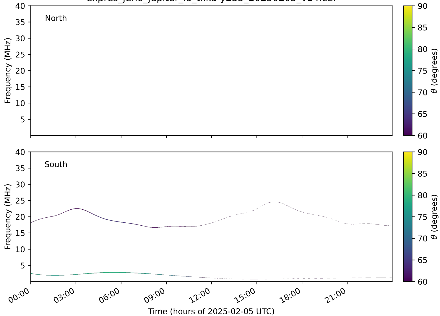
expres_juno_jupiter_io_txka-y235_20250205_v14.cdf
