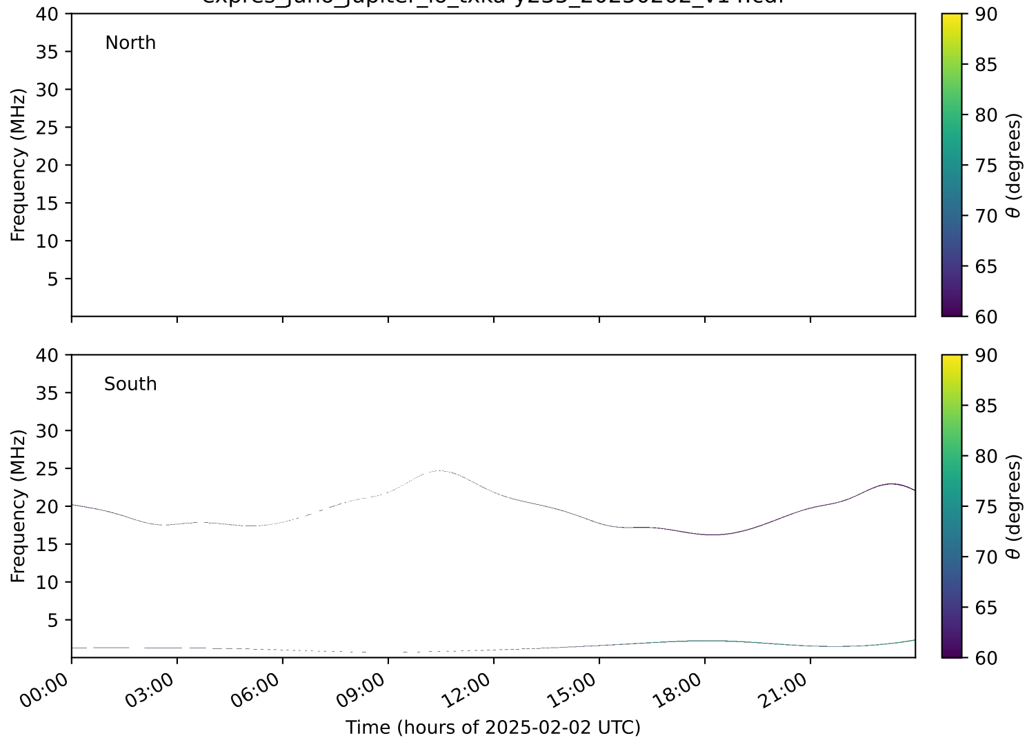
expres_juno_jupiter_io_txka-y235_20250202_v14.cdf
