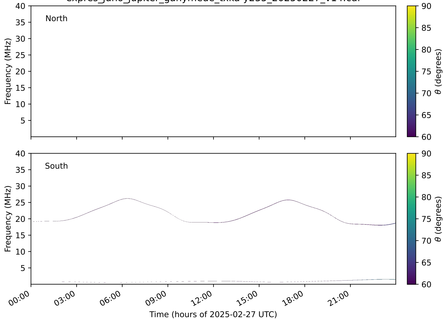
expres_juno_jupiter_ganymede_txka-y235_20250227_v14.cdf
