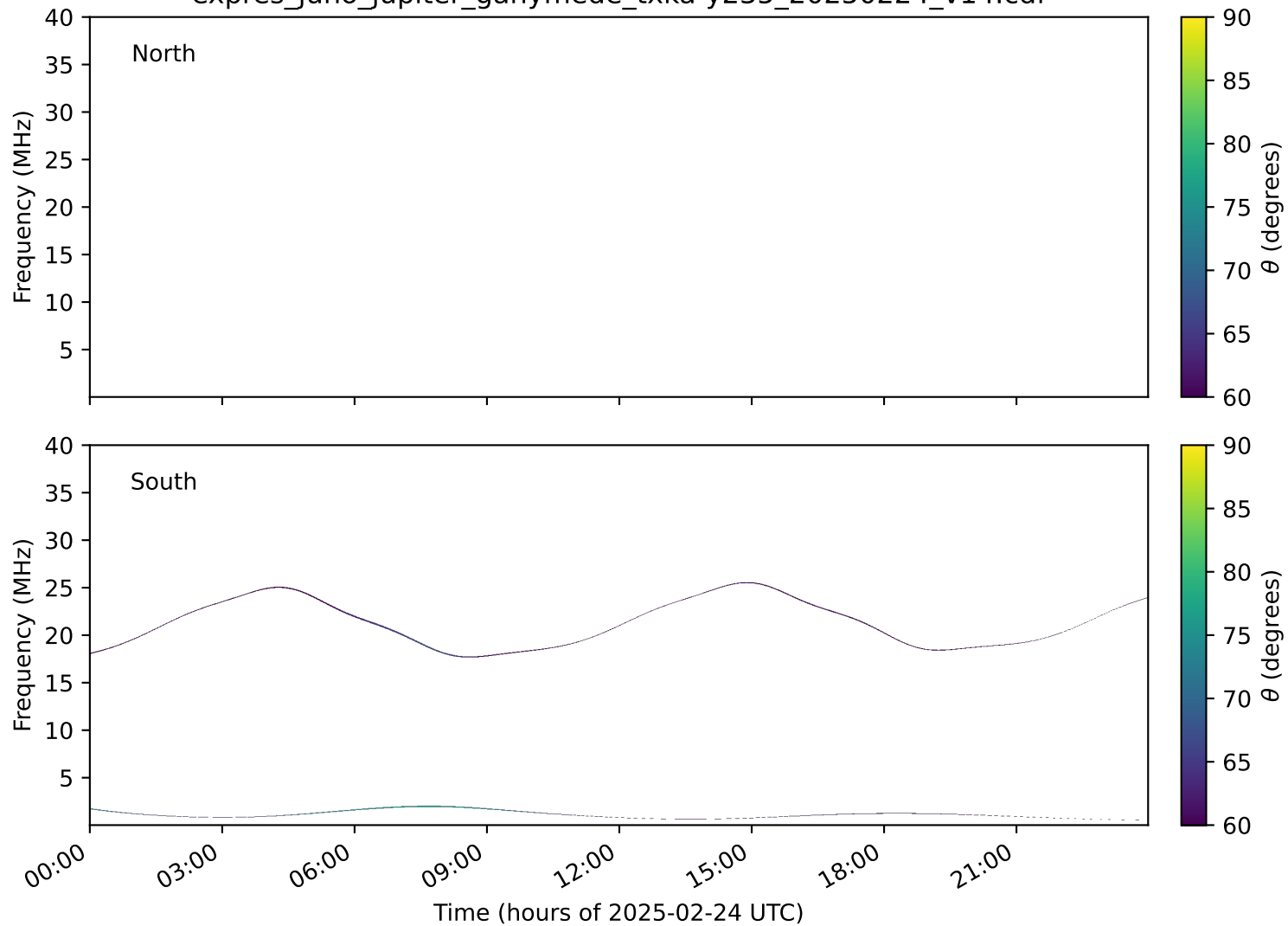
expres_juno_jupiter_ganymede_txka-y235_20250224_v14.cdf
