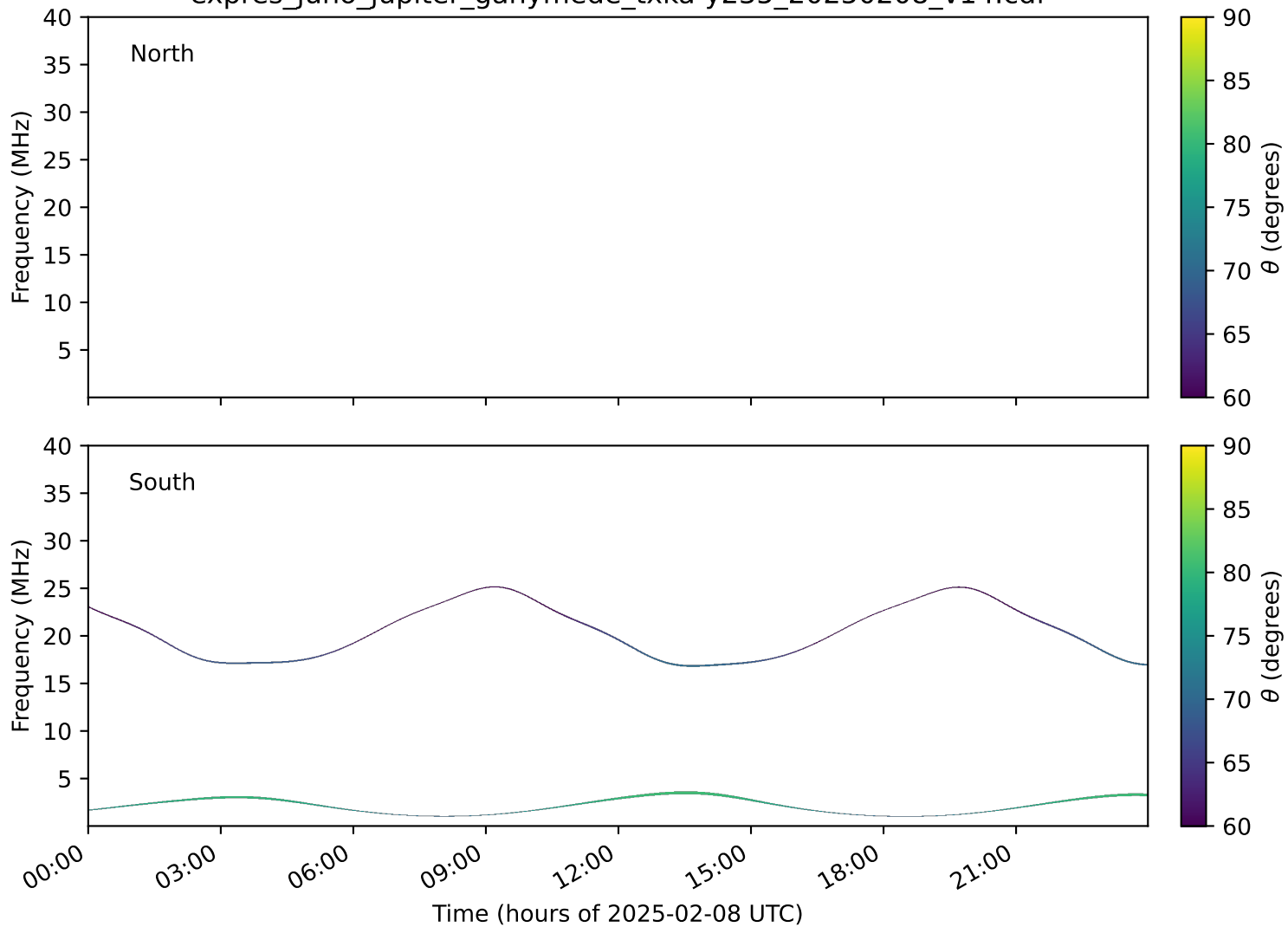
expres_juno_jupiter_ganymede_txka-y235_20250208_v14.cdf
