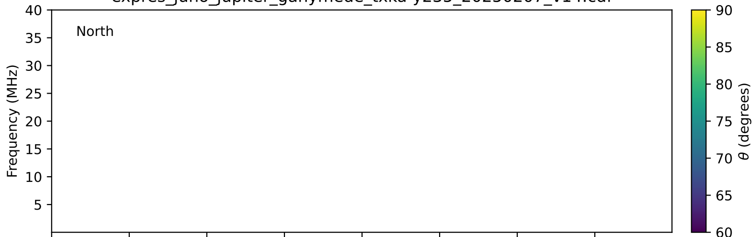
expres_juno_jupiter_ganymede_txka-y235_20250207_v14.cdf
