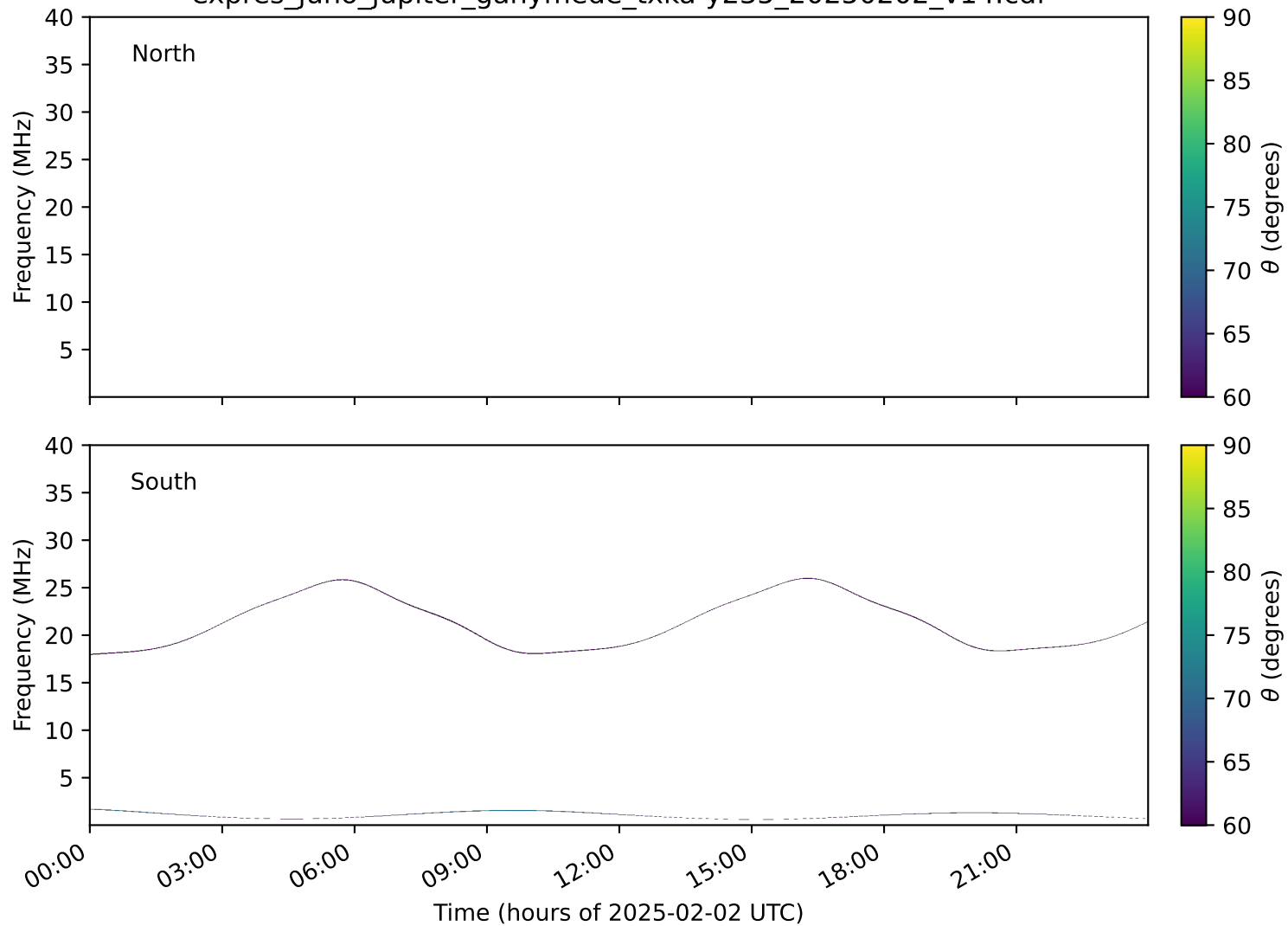
expres_juno_jupiter_ganymede_txka-y235_20250202_v14.cdf
