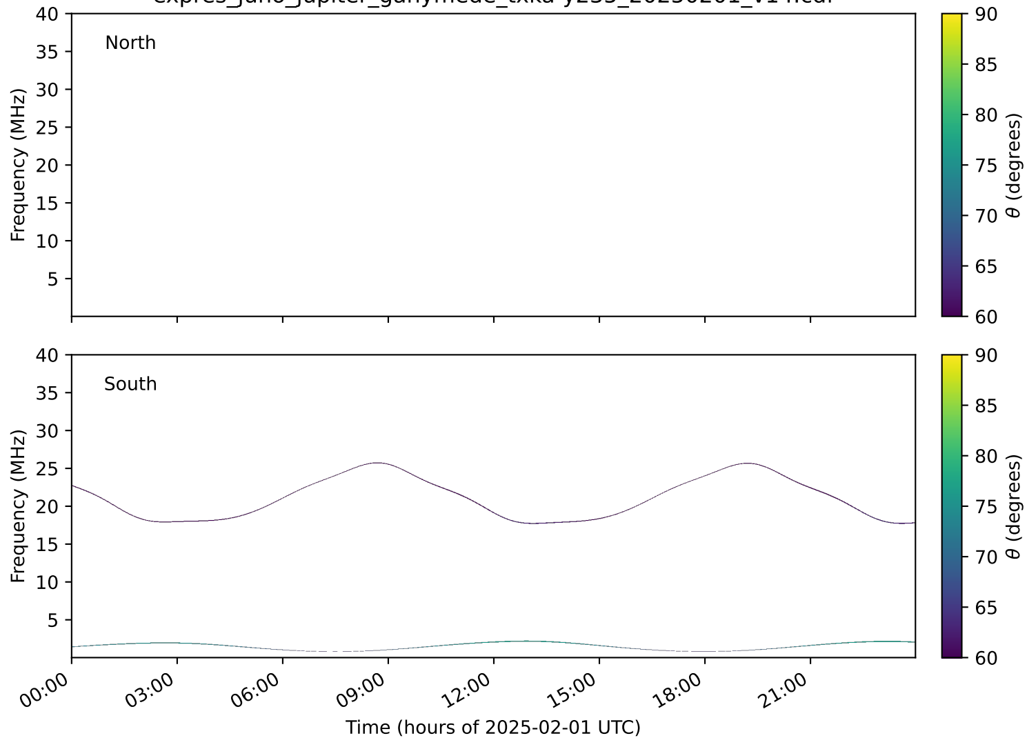
expres_juno_jupiter_ganymede_txka-y235_20250201_v14.cdf
