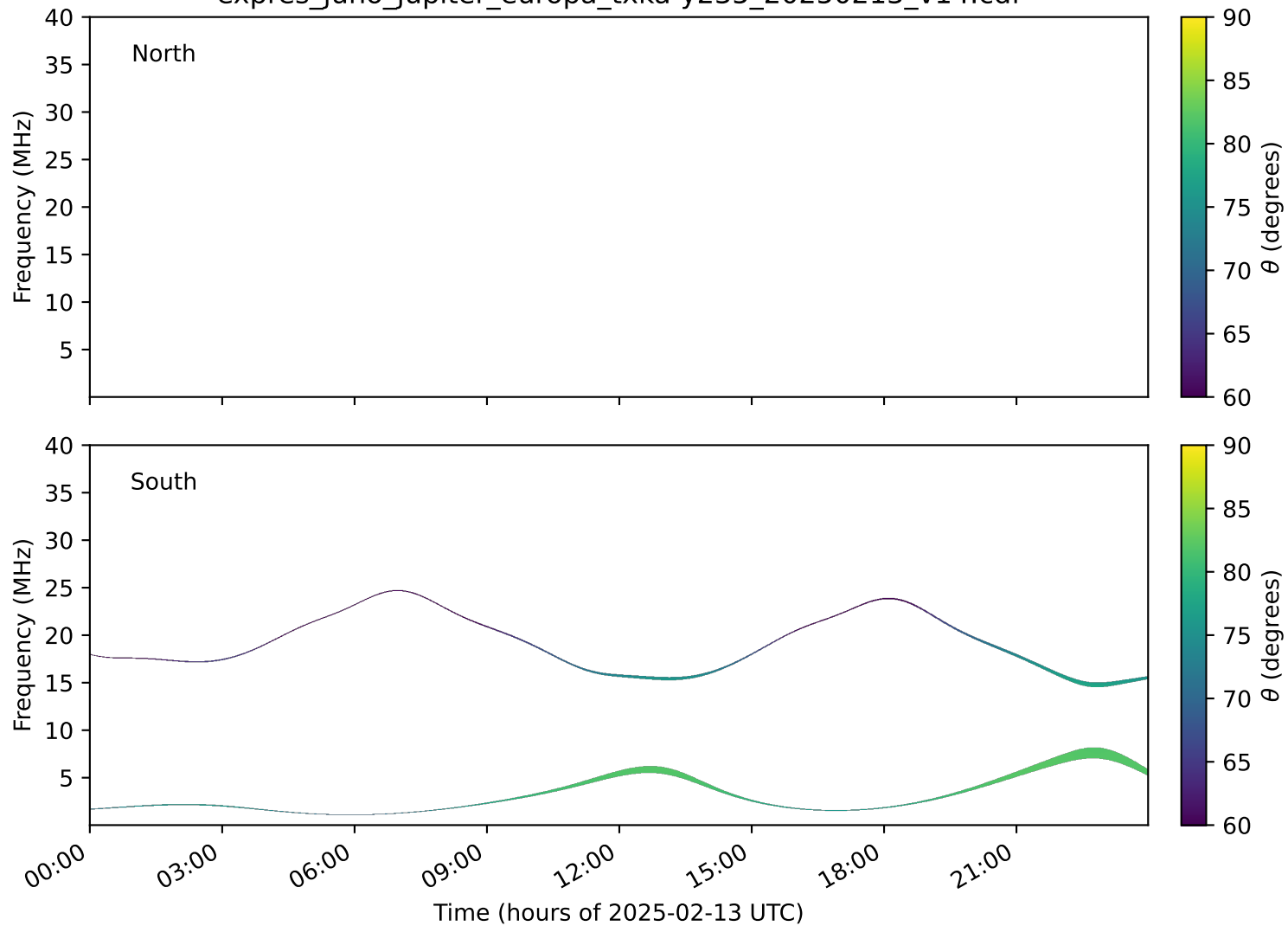
expres_juno_jupiter_europa_txka-y235_20250213_v14.cdf
