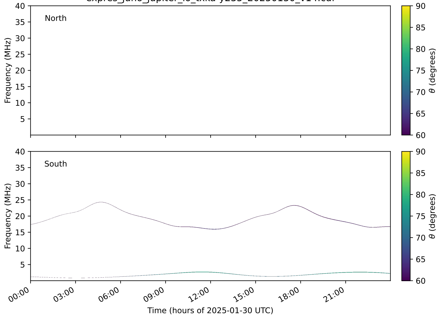
expres_juno_jupiter_io_txka-y235_20250130_v14.cdf
