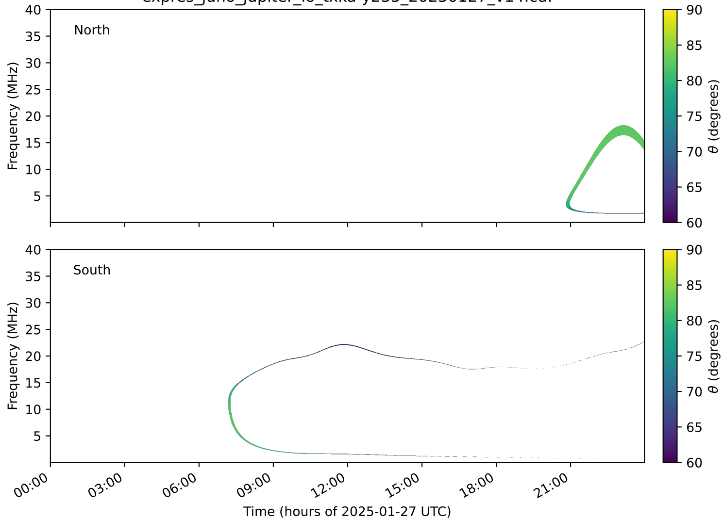
expres_juno_jupiter_io_txka-y235_20250127_v14.cdf
