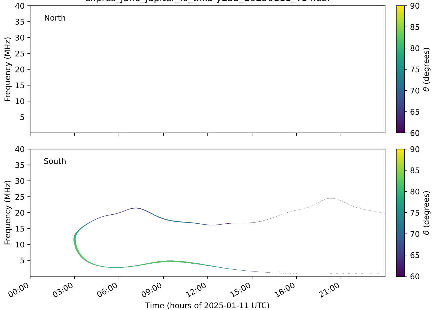
expres_juno_jupiter_io_txka-y235_20250111_v14.cdf
