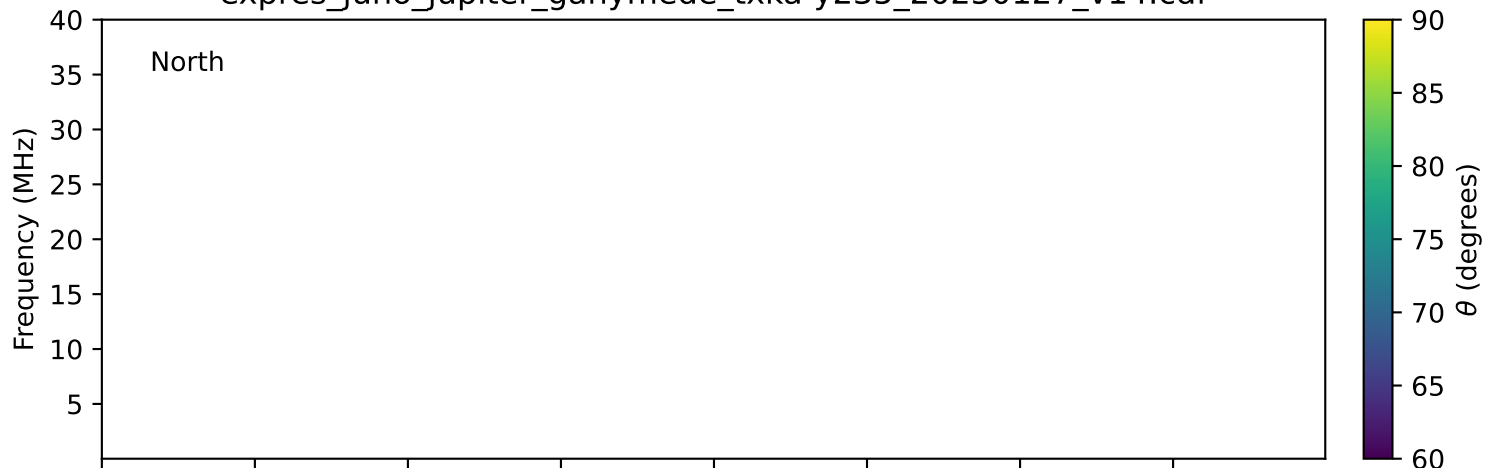
expres_juno_jupiter_ganymede_txka-y235_20250127_v14.cdf
