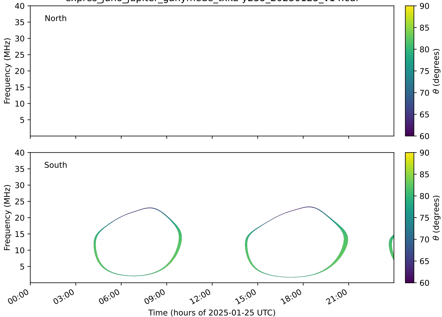
expres_juno_jupiter_ganymede_txka-y235_20250125_v14.cdf
