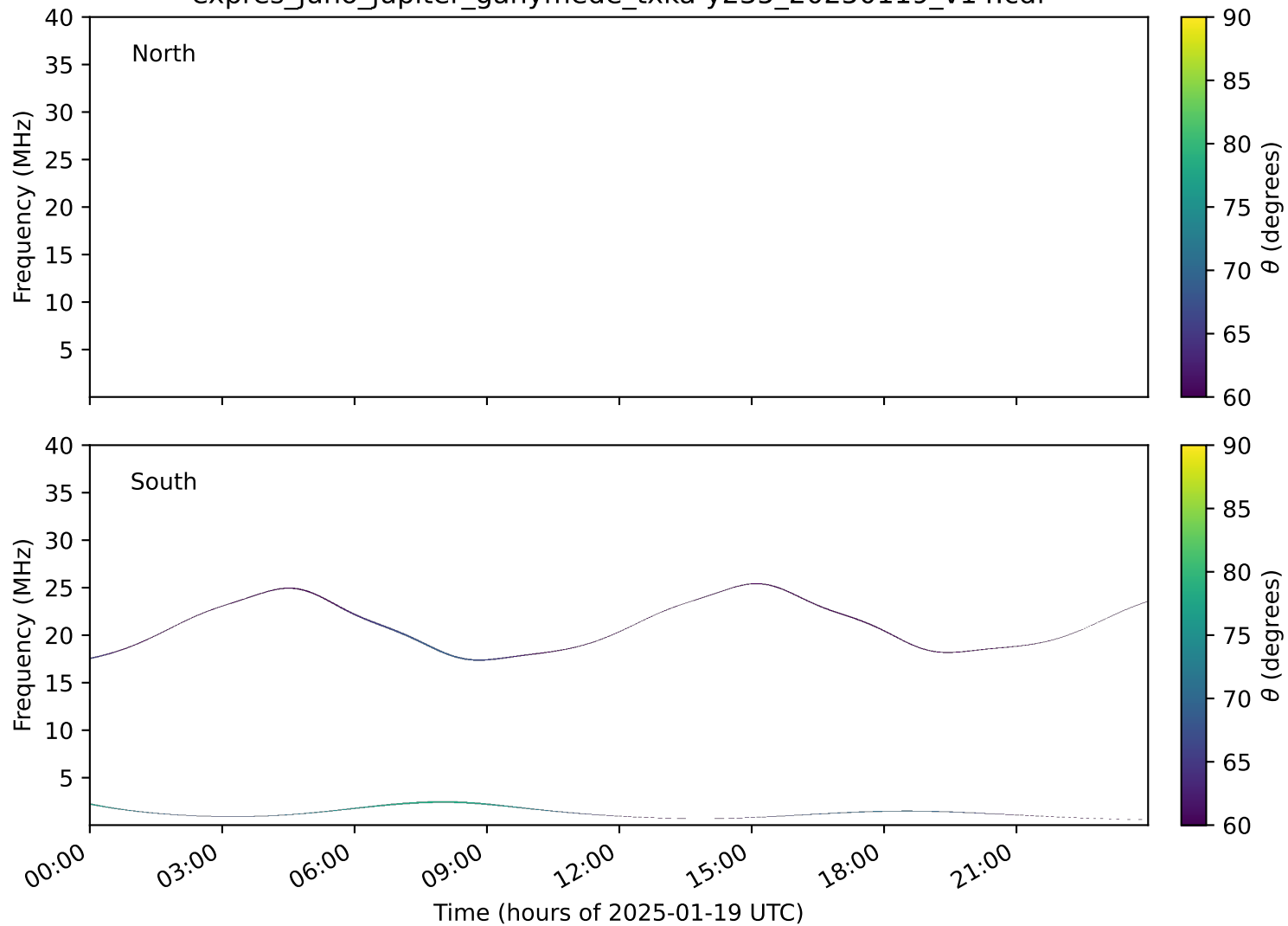
expres_juno_jupiter_ganymede_txka-y235_20250119_v14.cdf
