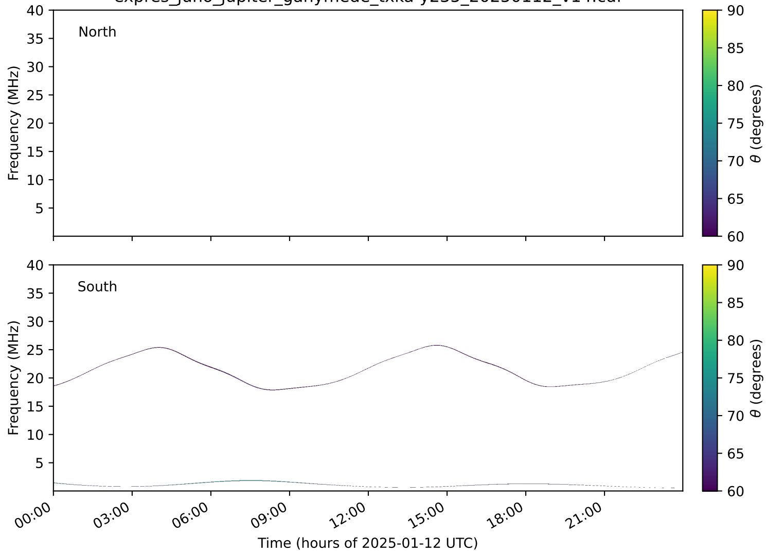
expres_juno_jupiter_ganymede_txka-y235_20250112_v14.cdf
