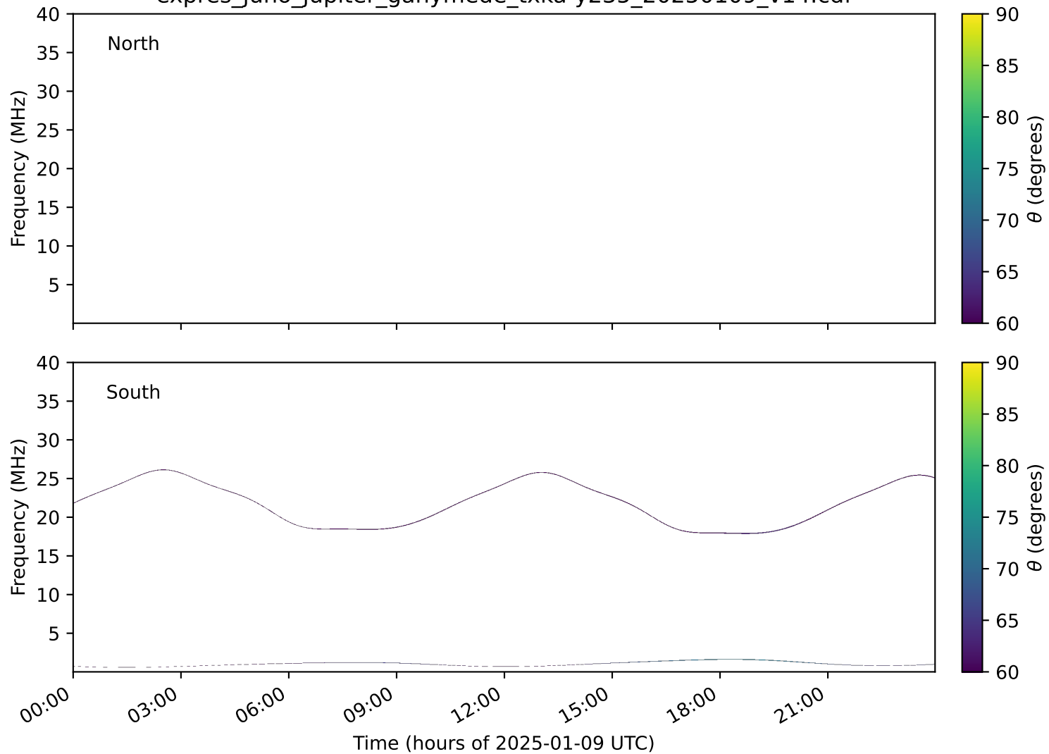
expres_juno_jupiter_ganymede_txka-y235_20250109_v14.cdf
