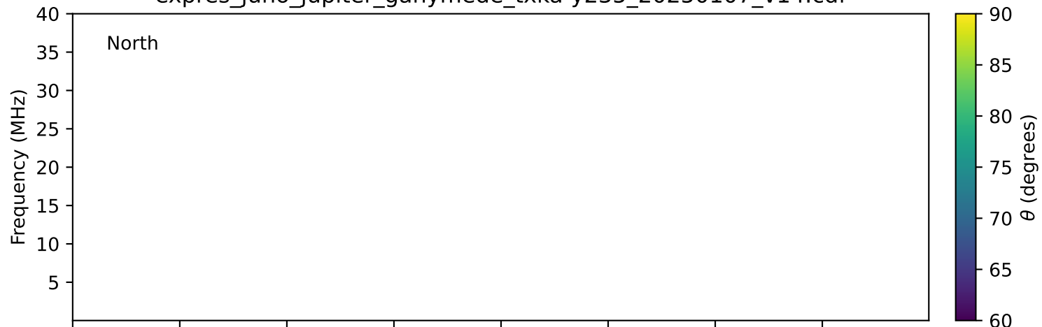
expres_juno_jupiter_ganymede_txka-y235_20250107_v14.cdf
