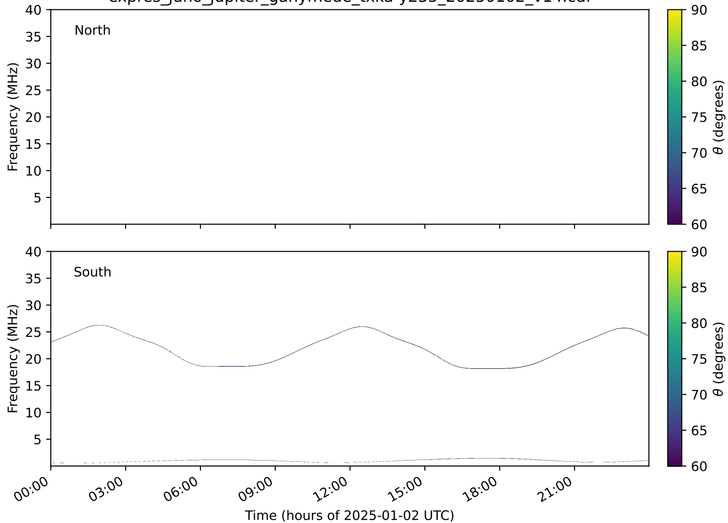
expres_juno_jupiter_ganymede_txka-y235_20250102_v14.cdf
