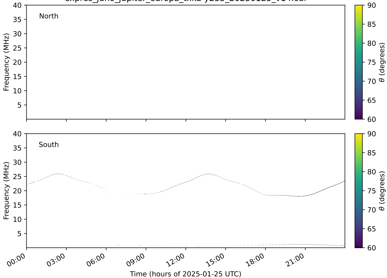
expres_juno_jupiter_europa_txka-y235_20250125_v14.cdf
