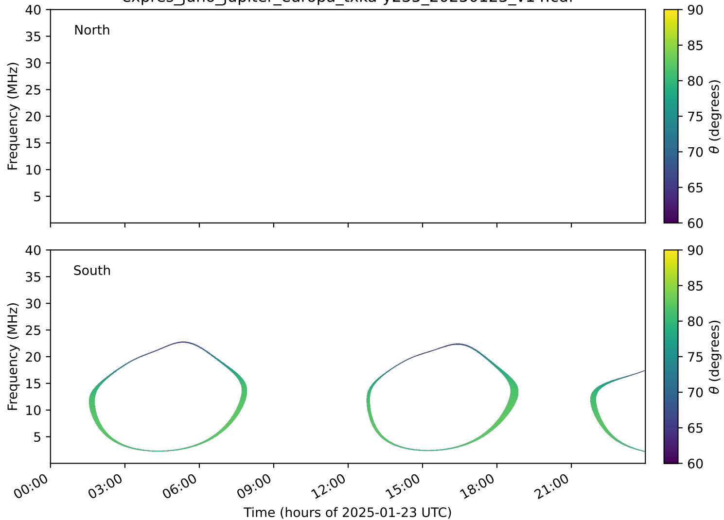
expres_juno_jupiter_europa_txka-y235_20250123_v14.cdf
