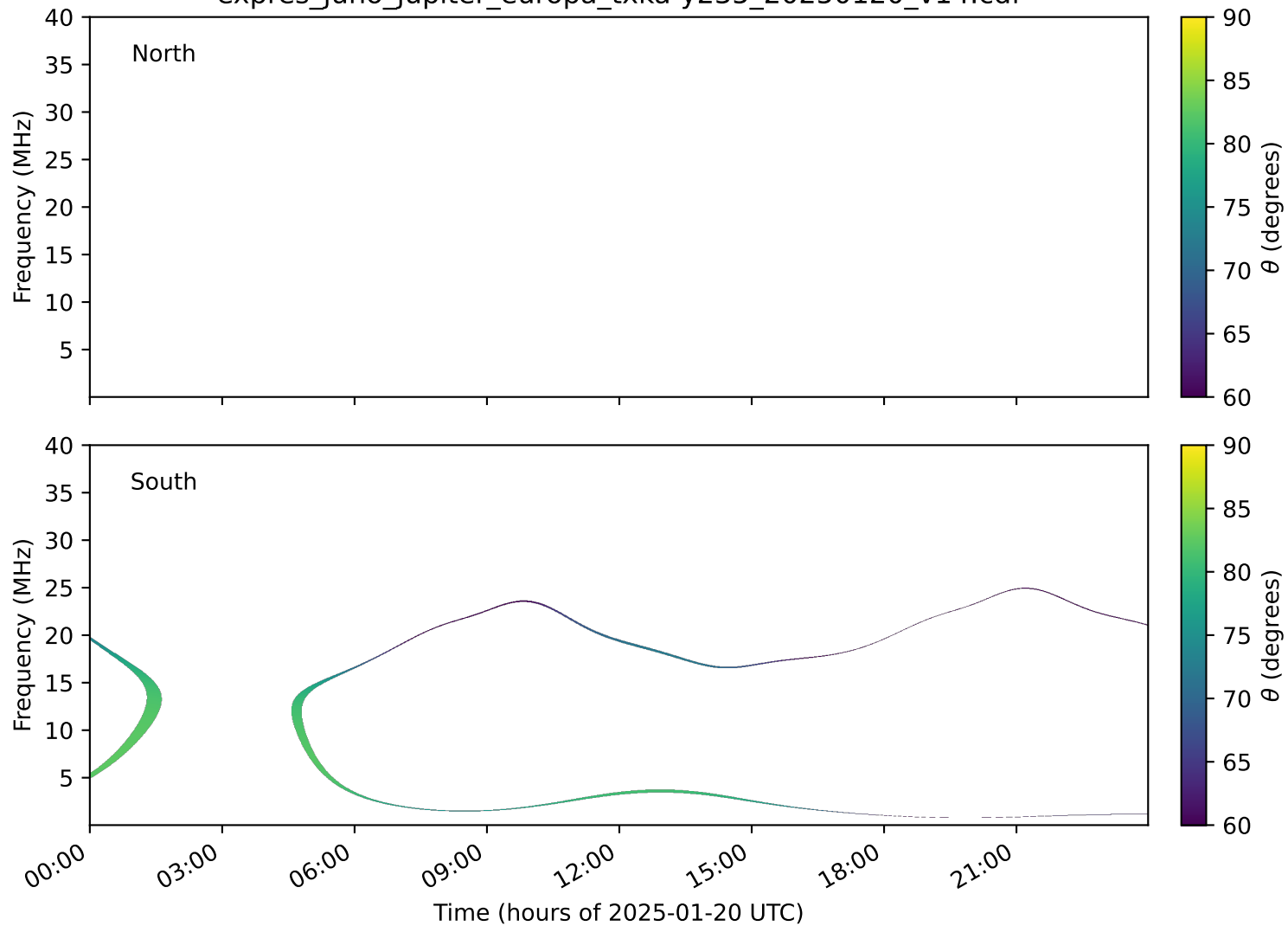
expres_juno_jupiter_europa_txka-y235_20250120_v14.cdf
