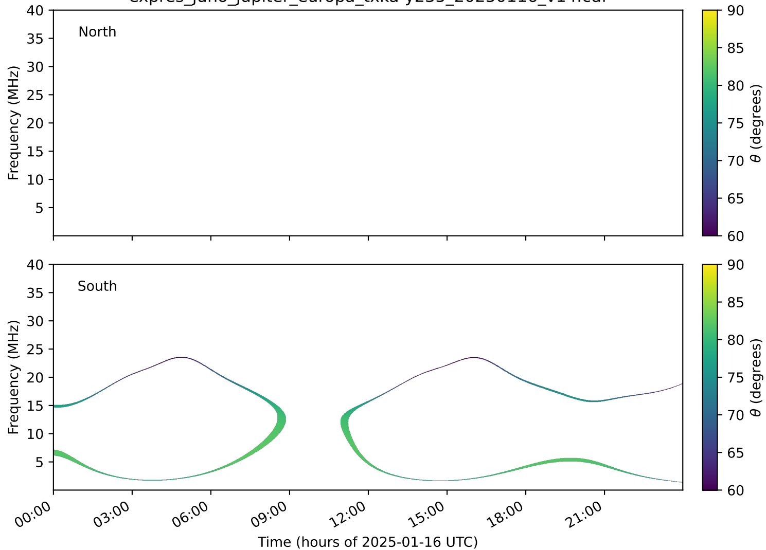
expres_juno_jupiter_europa_txka-y235_20250116_v14.cdf
