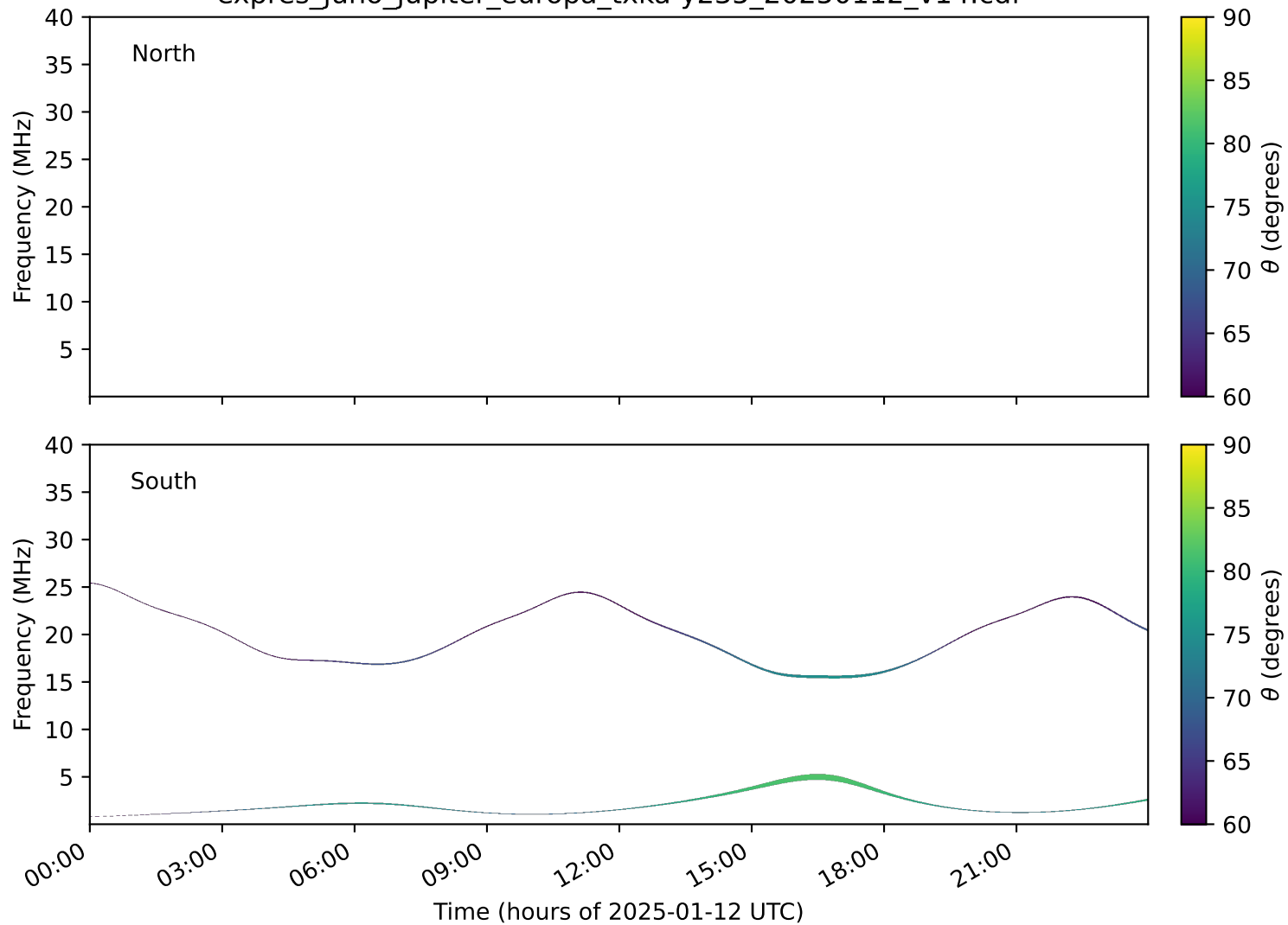
expres_juno_jupiter_europa_txka-y235_20250112_v14.cdf
