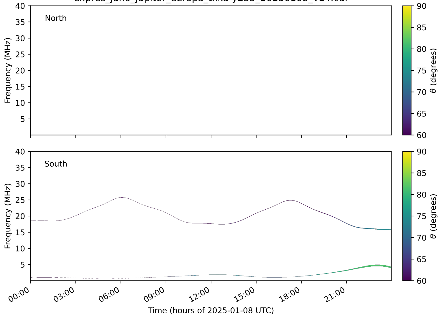
expres_juno_jupiter_europa_txka-y235_20250108_v14.cdf
