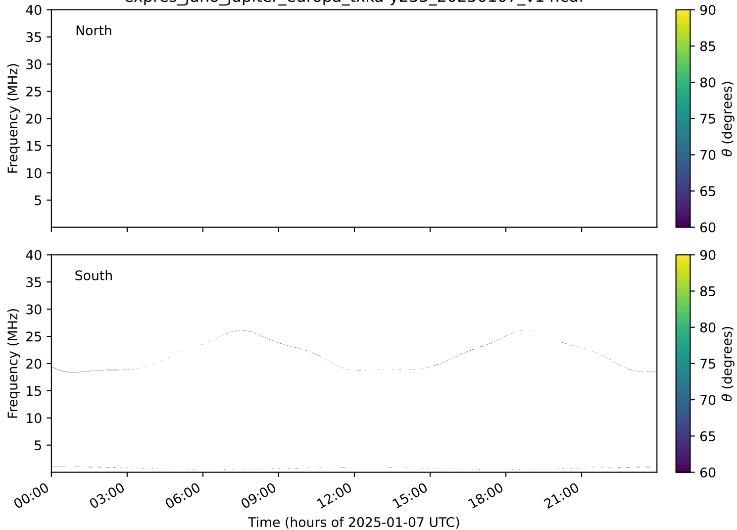
expres_juno_jupiter_europa_txka-y235_20250107_v14.cdf
