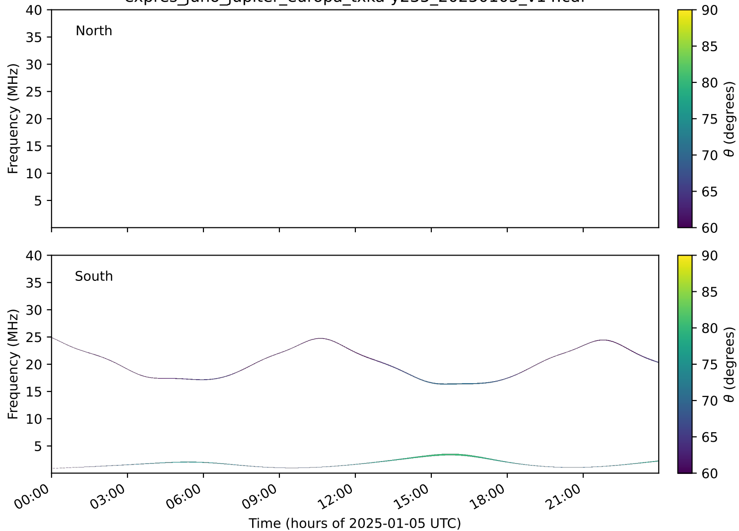
expres_juno_jupiter_europa_txka-y235_20250105_v14.cdf
