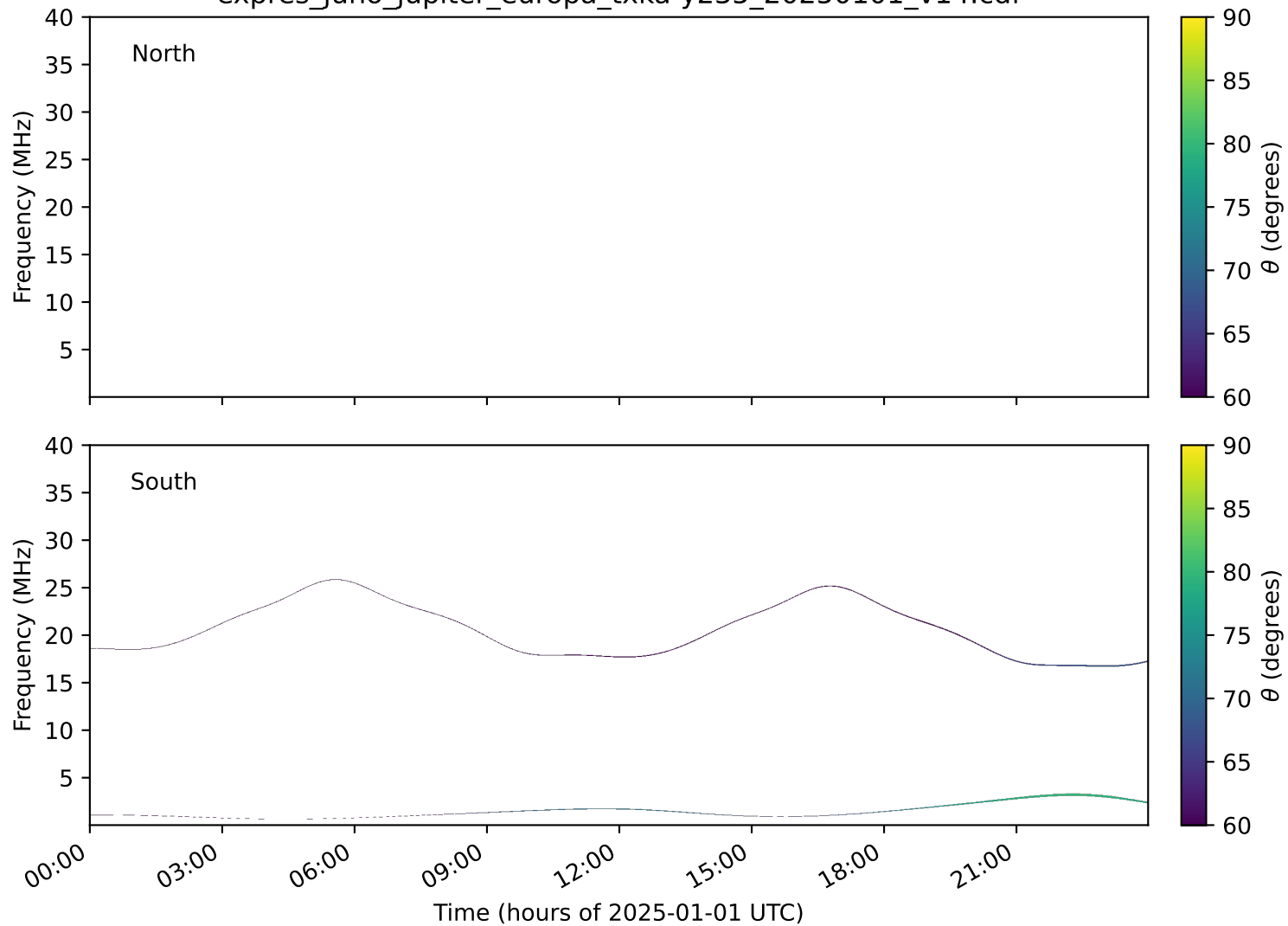
expres_juno_jupiter_europa_txka-y235_20250101_v14.cdf
