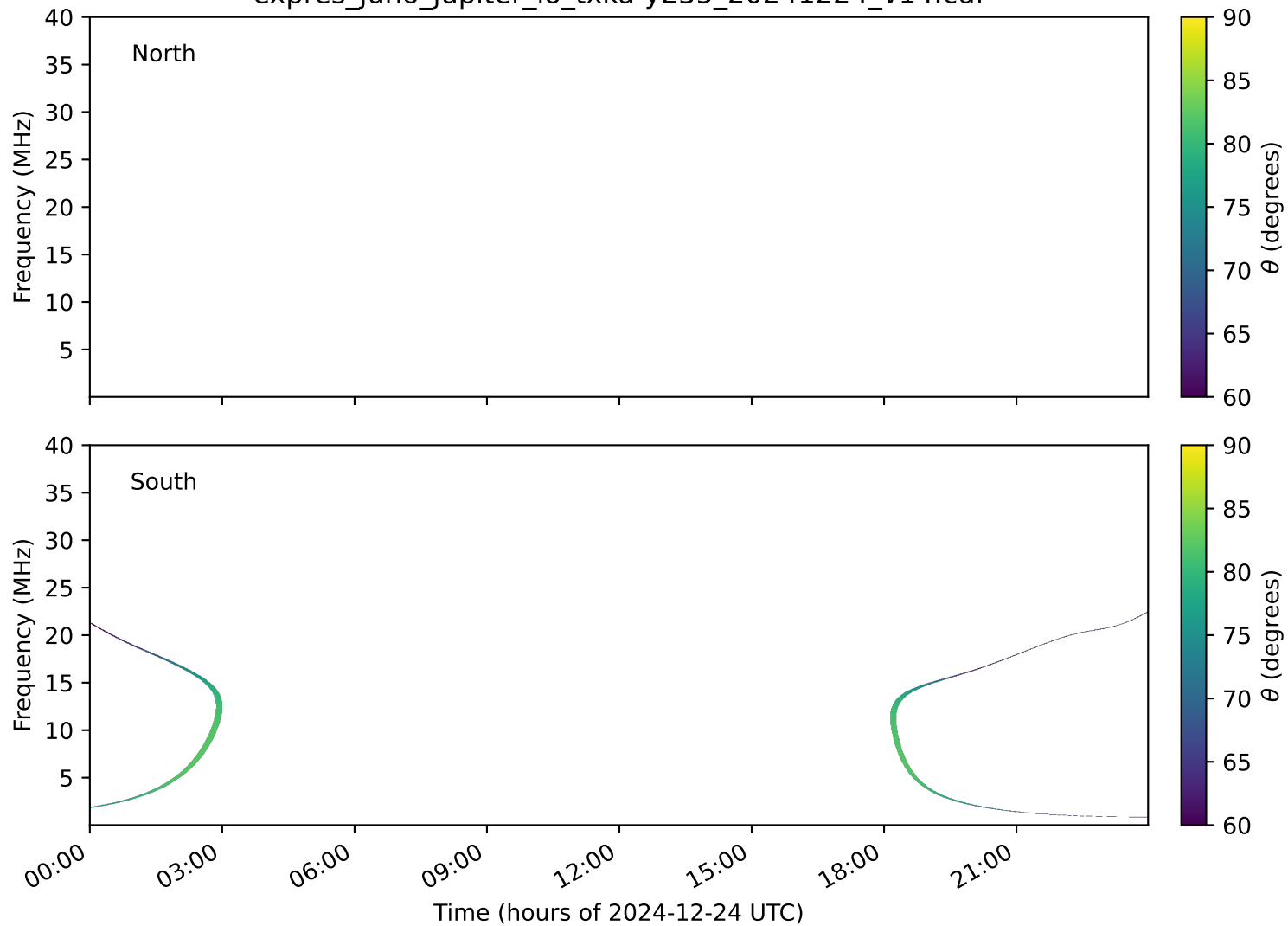
expres_juno_jupiter_io_txka-y235_20241224_v14.cdf
