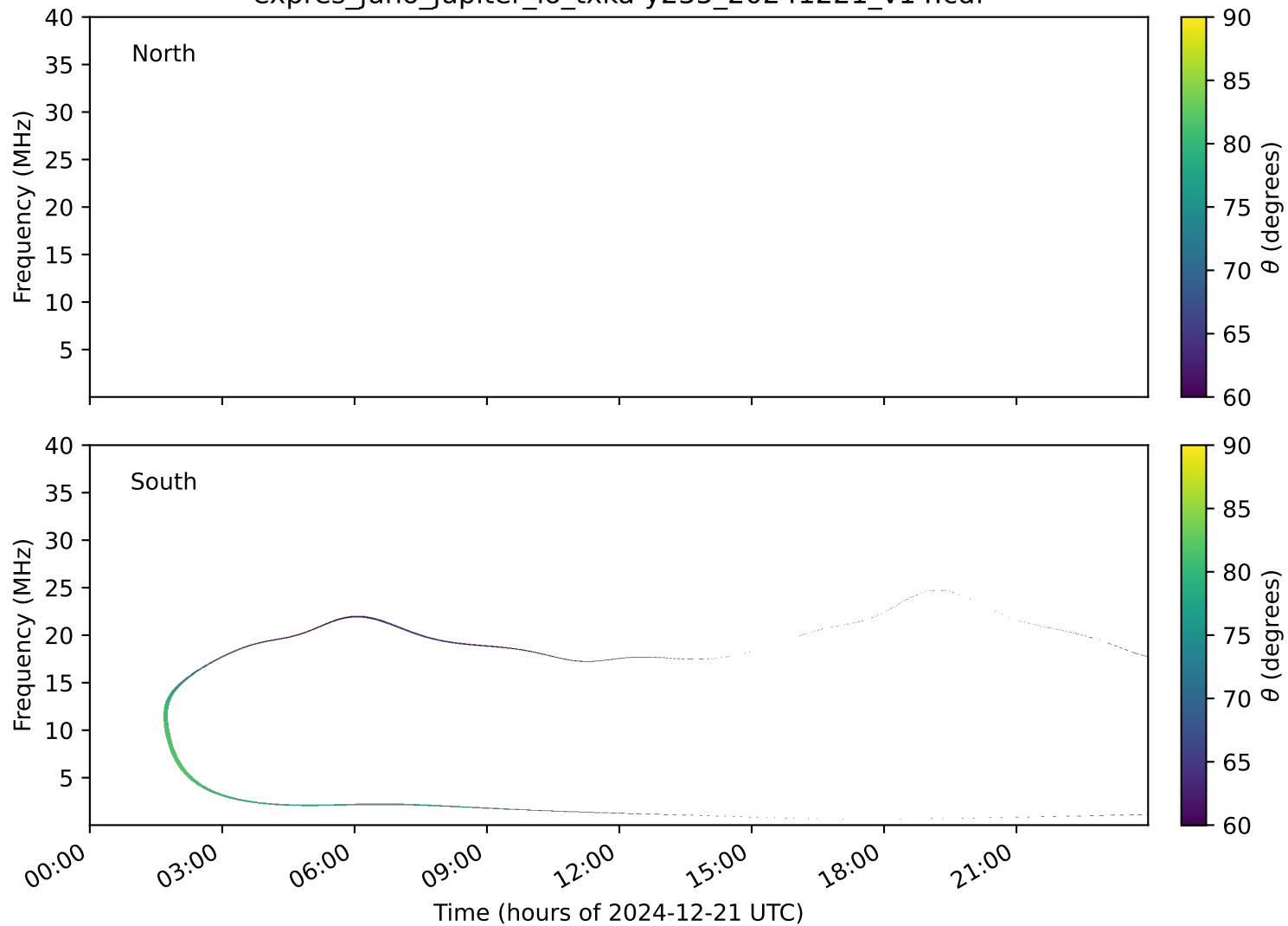
expres_juno_jupiter_io_txka-y235_20241221_v14.cdf
