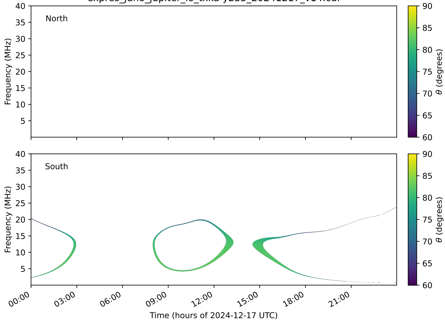
expres_juno_jupiter_io_txka-y235_20241217_v14.cdf
