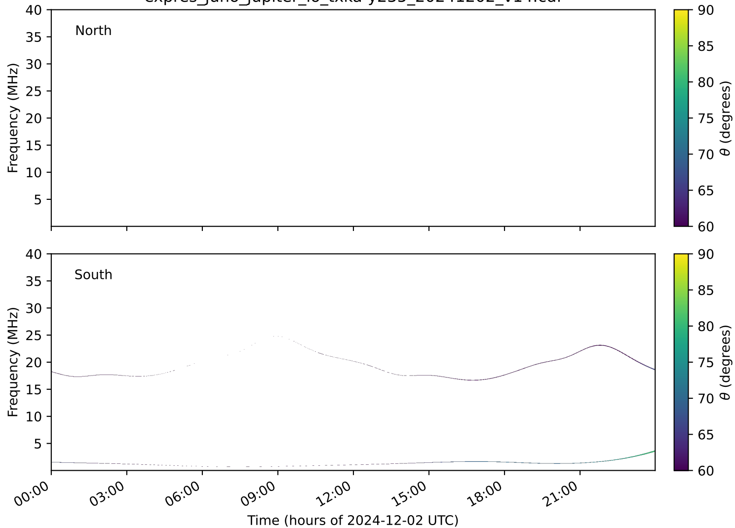
expres_juno_jupiter_io_txka-y235_20241202_v14.cdf
