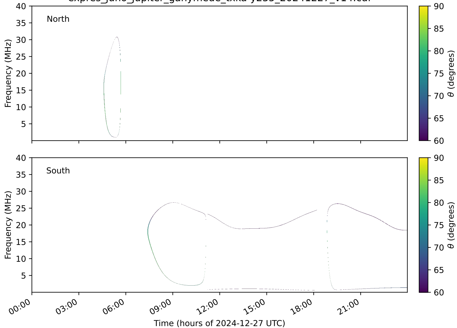
expres_juno_jupiter_ganymede_txka-y235_20241227_v14.cdf
