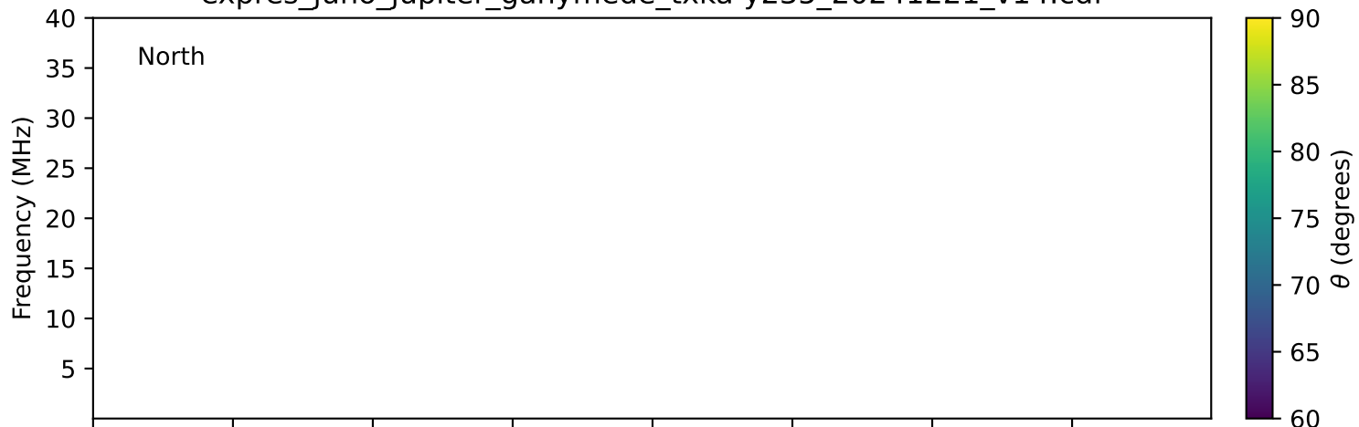
expres_juno_jupiter_ganymede_txka-y235_20241221_v14.cdf
