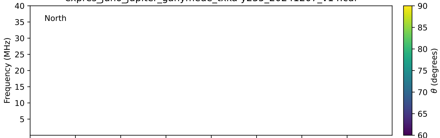
expres_juno_jupiter_ganymede_txka-y235_20241207_v14.cdf
