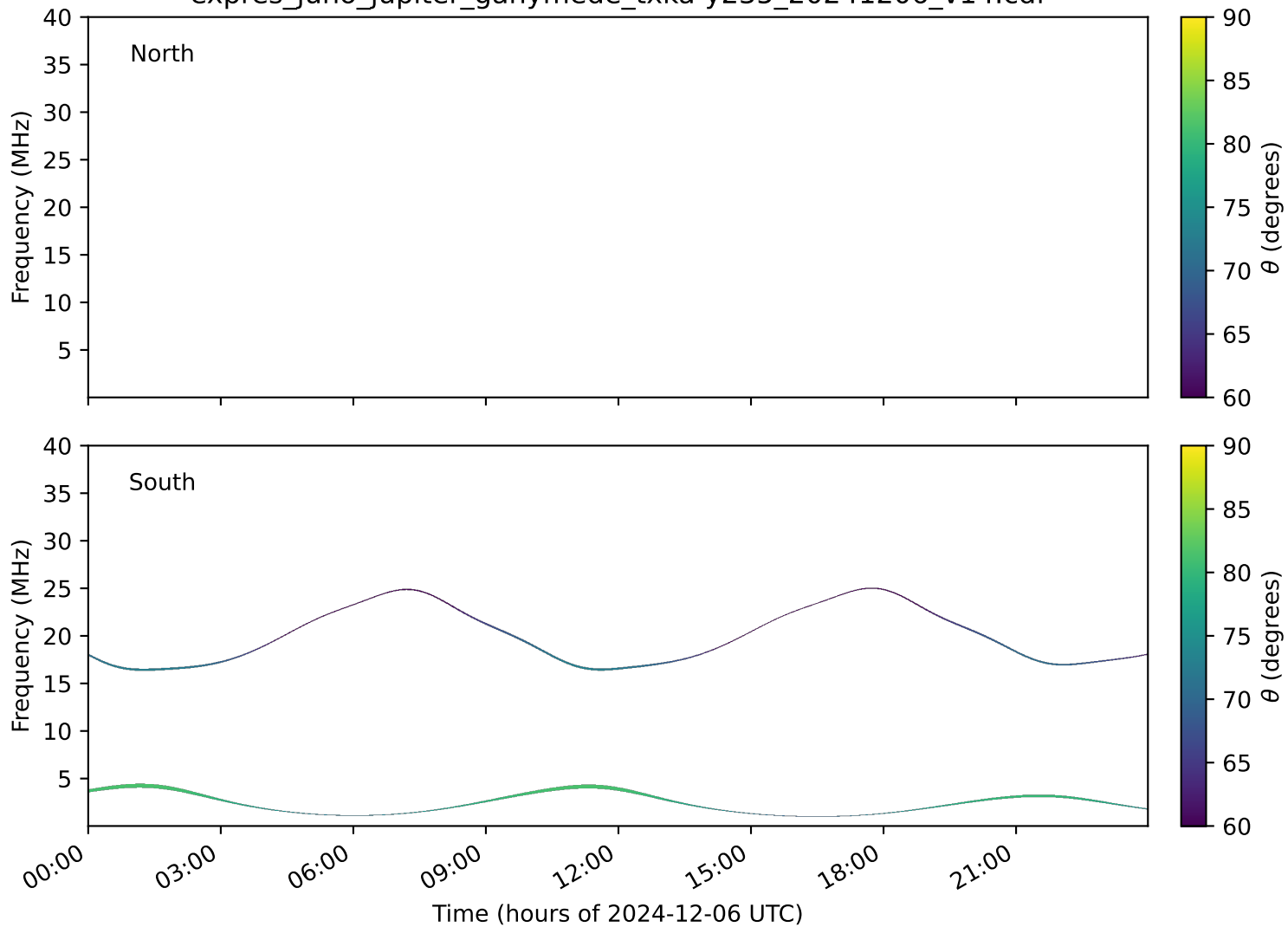
expres_juno_jupiter_ganymede_txka-y235_20241206_v14.cdf
