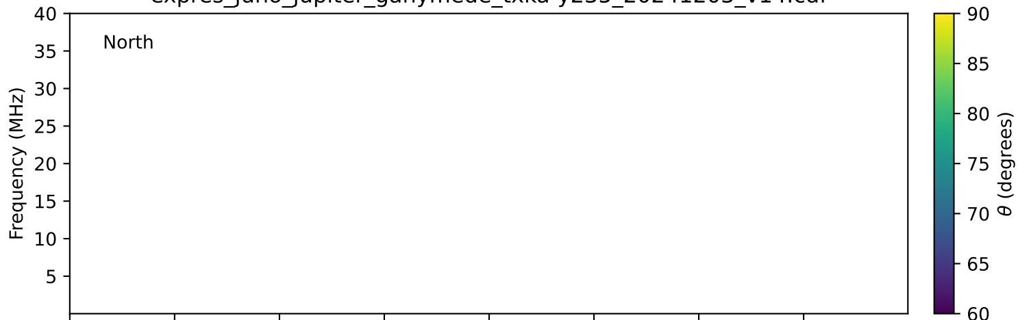
expres_juno_jupiter_ganymede_txka-y235_20241203_v14.cdf
