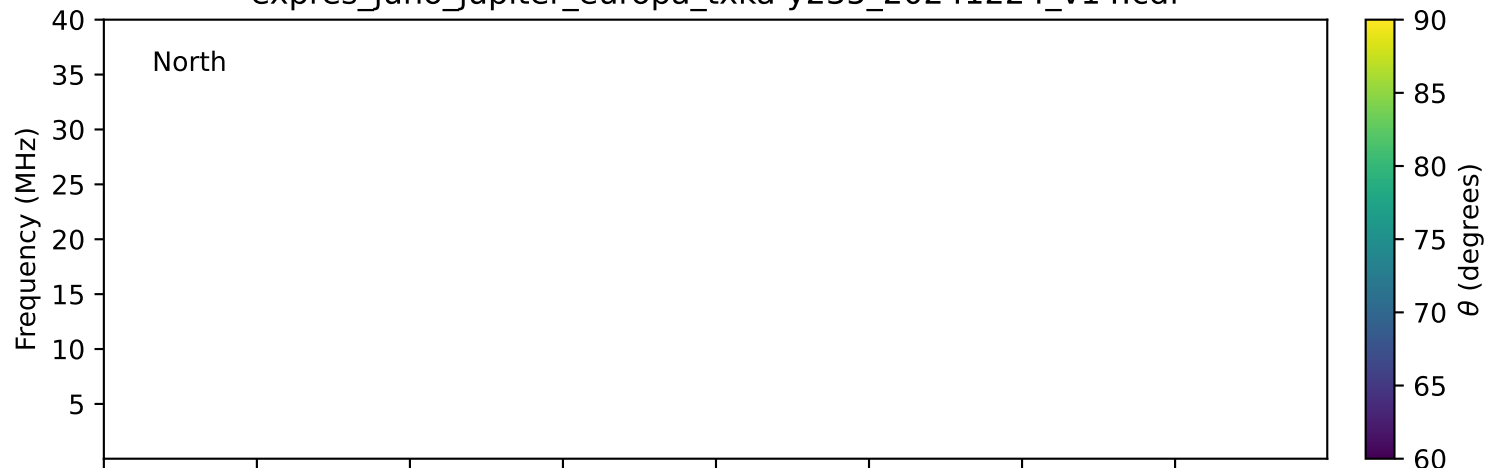
expres_juno_jupiter_europa_txka-y235_20241224_v14.cdf
