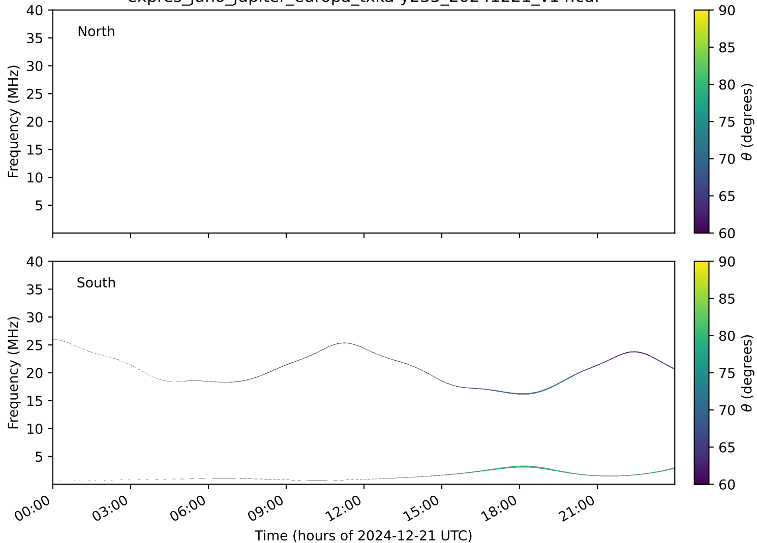
expres_juno_jupiter_europa_txka-y235_20241221_v14.cdf
