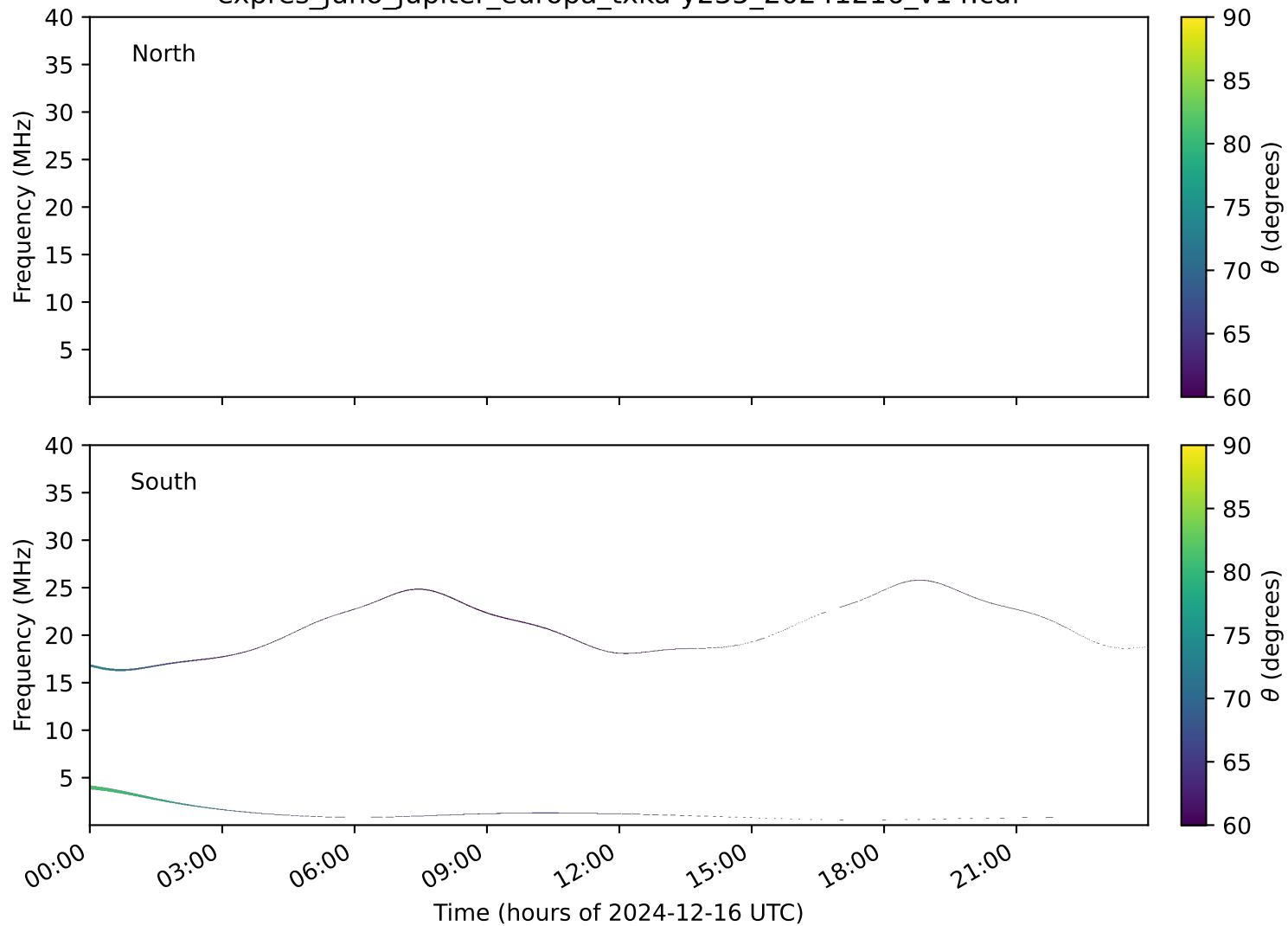
expres_juno_jupiter_europa_txka-y235_20241216_v14.cdf
