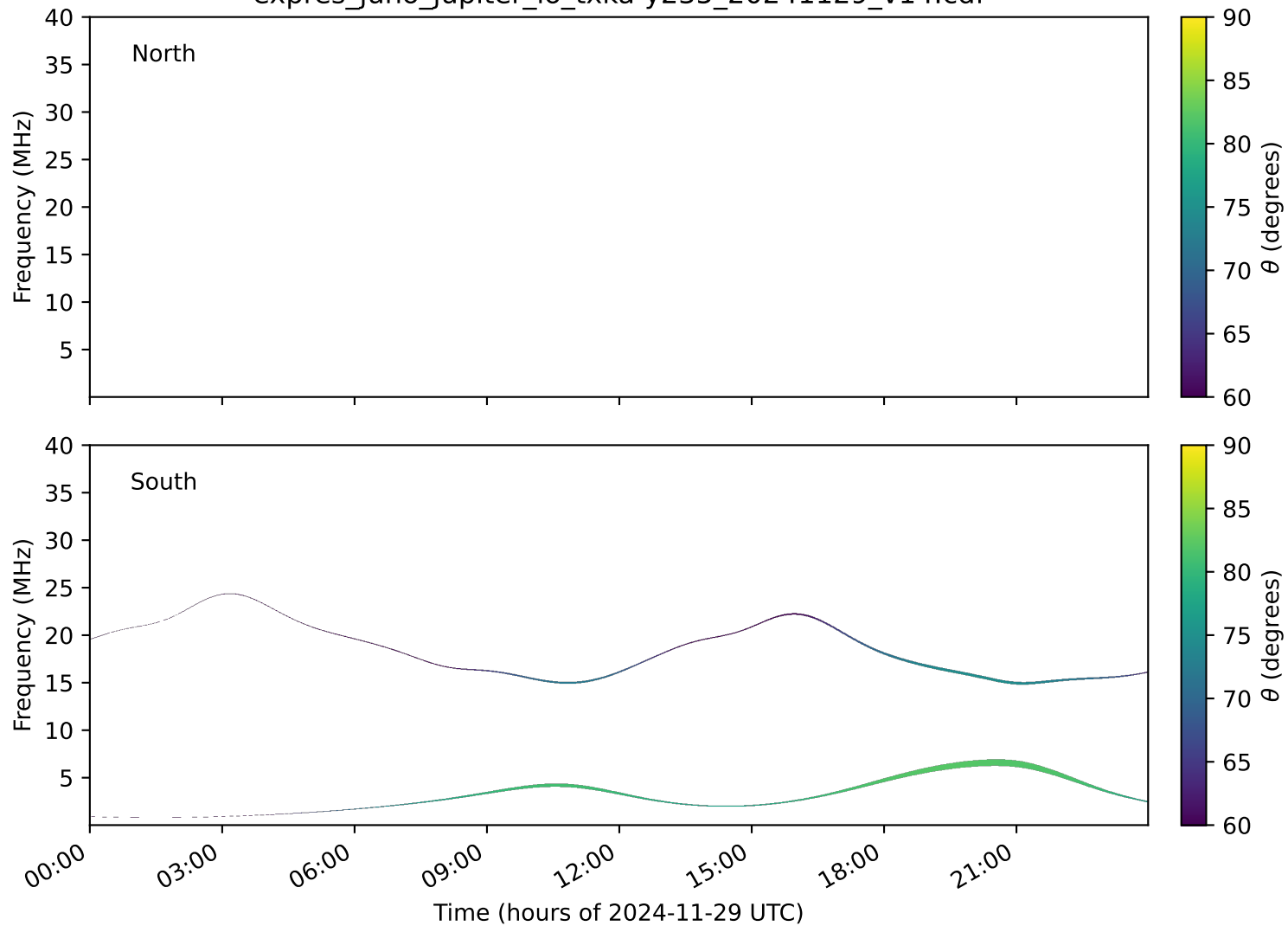
expres_juno_jupiter_io_txka-y235_20241129_v14.cdf
